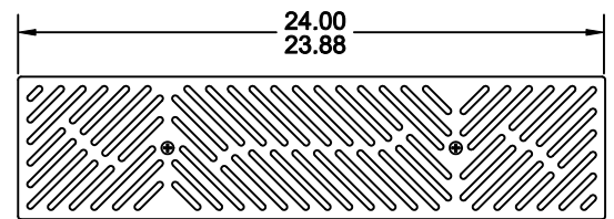
TOP VIEW (GRATE ONLY- 2 REQ'D)
